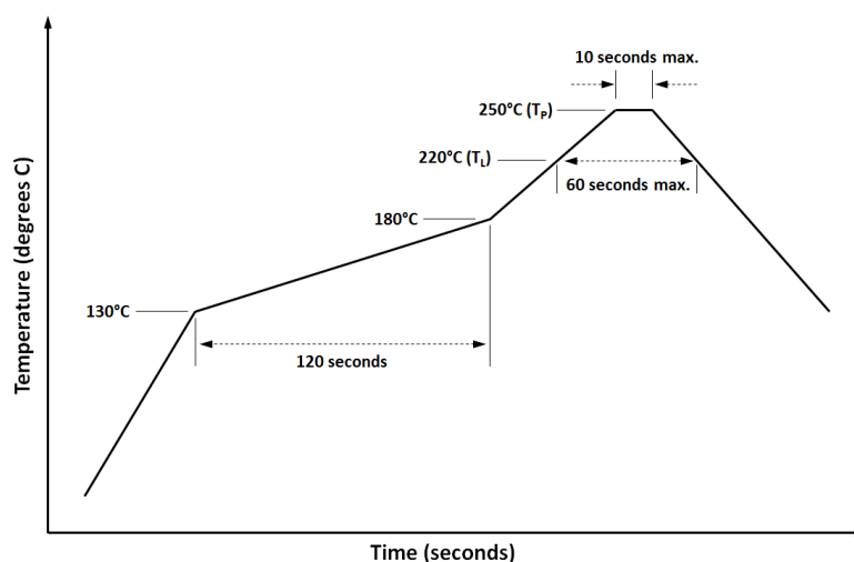
Figure 5 - Recommended solder reflow profile
